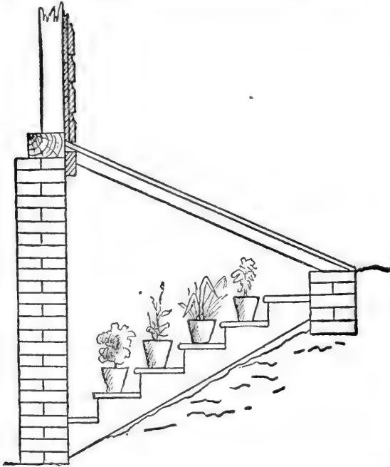
FIG. 118. CELLAR-WAY CONSERVATORY ( Section ).
